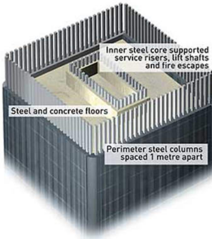
Technical diagram of the twin towers
