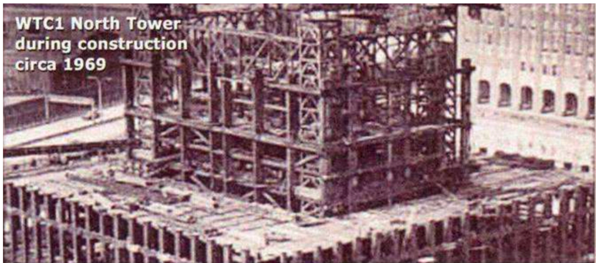
A photo of the building under construction in 1969 - steel structure in the core of the building.
